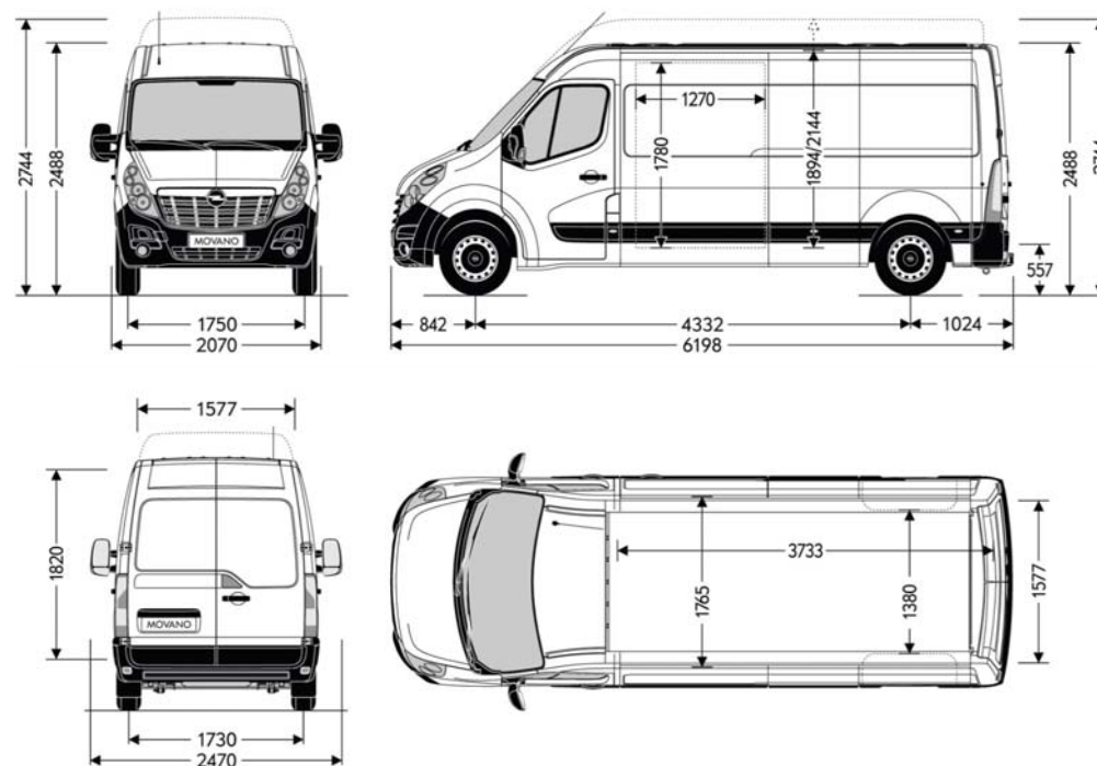
Opel Movano Van FWD L3H2-H3
